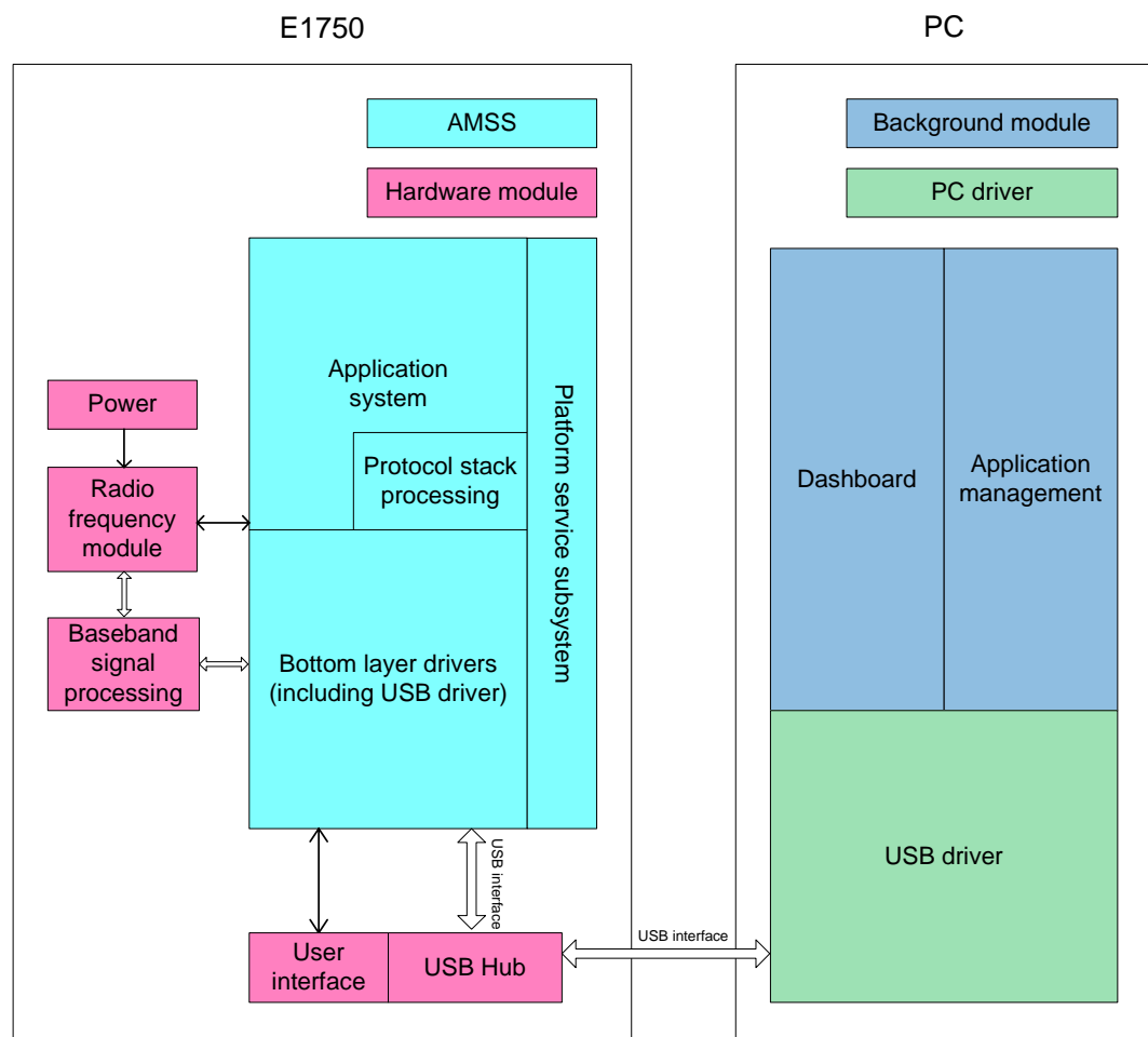
Figure 4-1 System architecture
